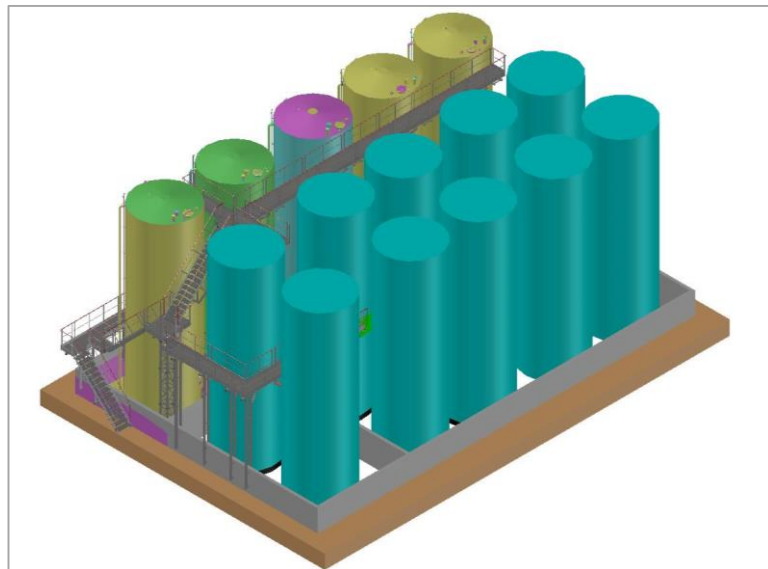
Staircases and gangways on « grease storage » tanks 3D representation
