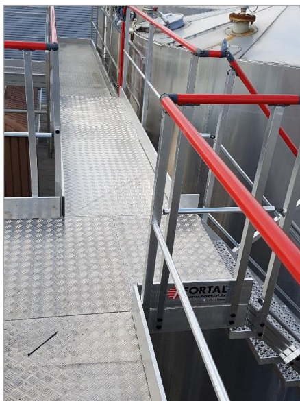
Platforms and gangways coating: flat sheet aluminum thickness 4.4 mm
