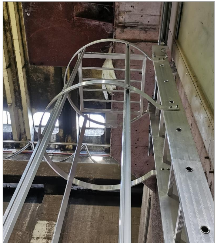
View on the low part of the « mobile » safety cage ladder
