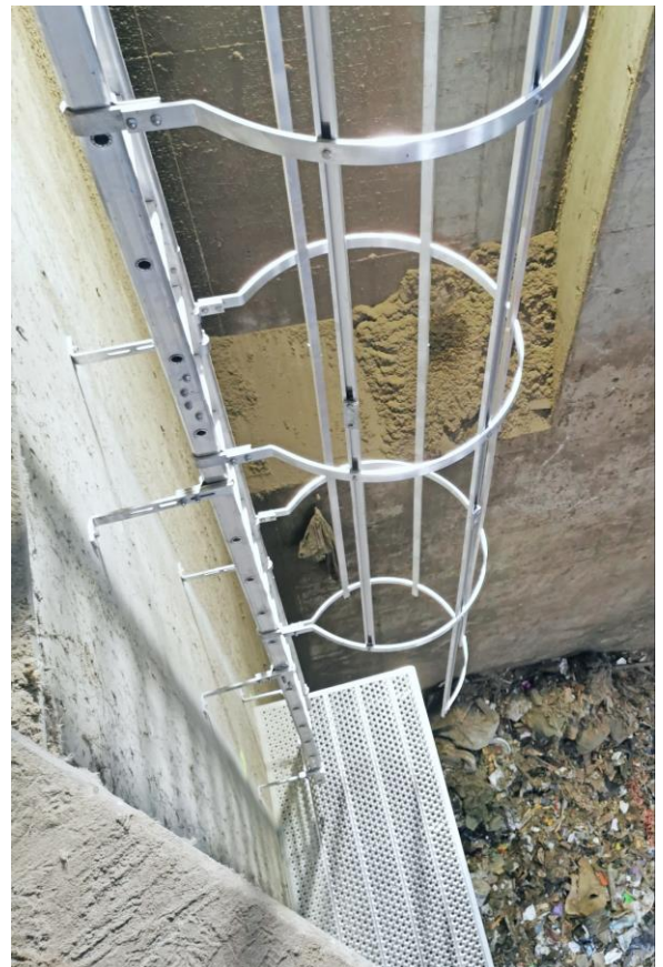
Installation of the safety cage ladders that allows safe access to the gangway from the top – height 5 700 mm – front exit with parapet bearing and safety gate on the upper part of safety cage ladder.
