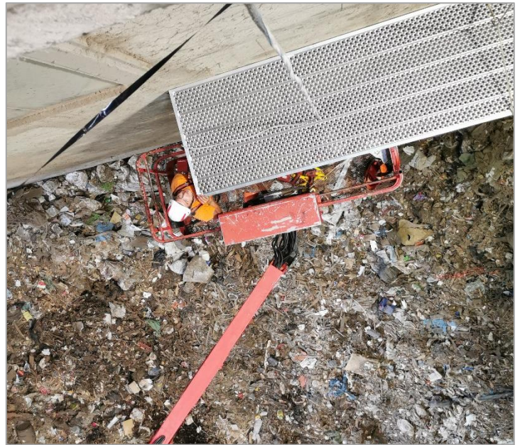
Installation of the gangway with support legs on concrete pit walls
