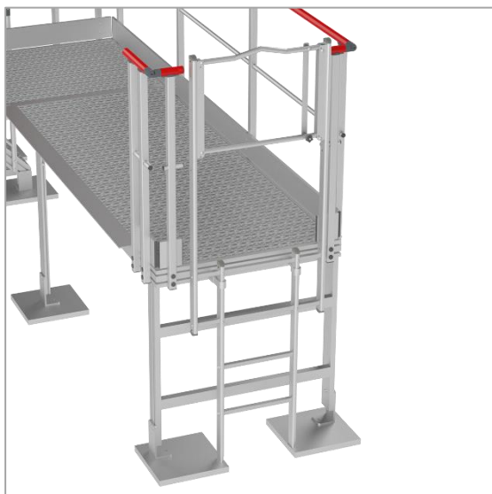
The platform is also accessible thanks a ladder with safety door at a platform end
